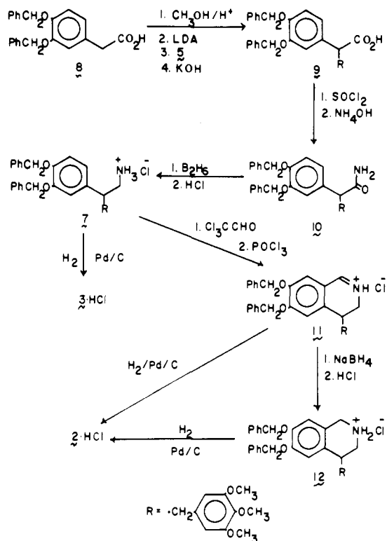
Scheme II
